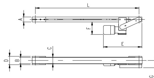
Type NB "LOW or STD model" End mounted drive unit
